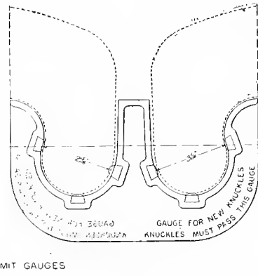
Fig. 5500. LIMIT GAGES FOR M. C. B. AUTOMATIC COUPLER Adopted in 1891.
